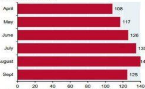
Persian Gulf expected peak temperatures in 2026 Temperature, Fahrenheit
